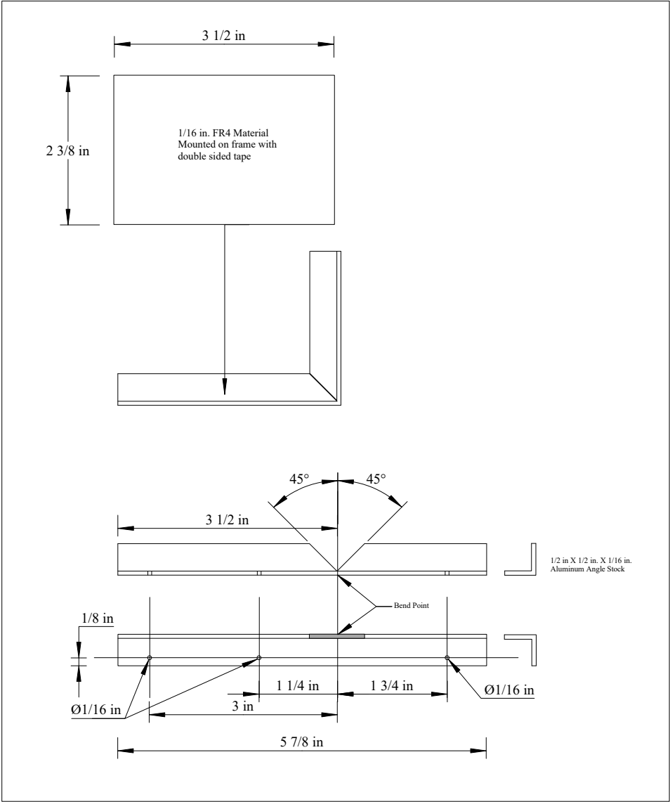
AC Power Safety Shield and Bracket
