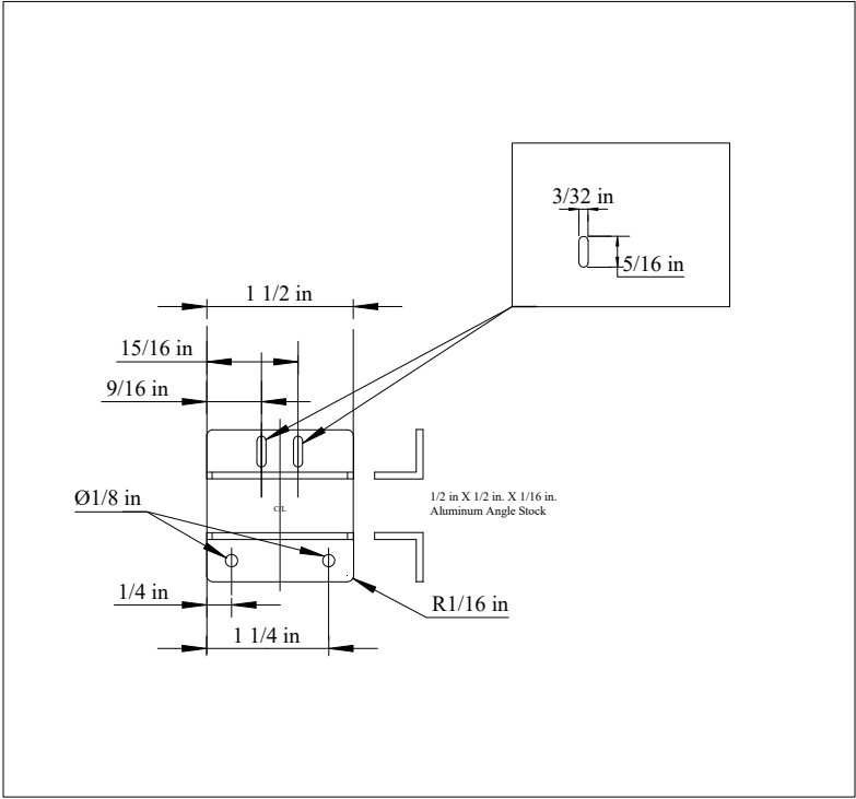
Fixture Closed Switch Bracket
